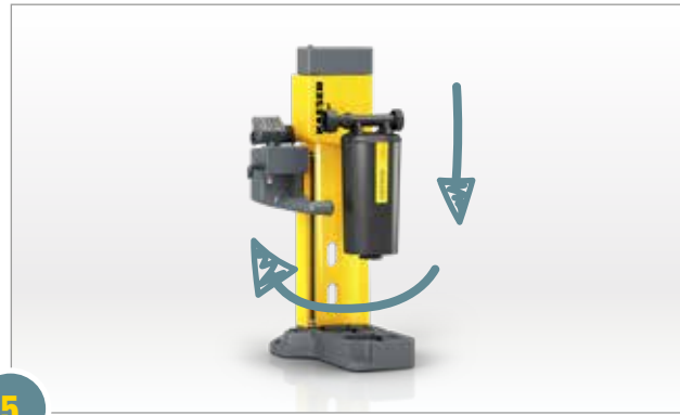
5 The new cartridges are inserted in reverse sequence accordingly. The screw connection clamping nuts are tightened – refer to step 2.
